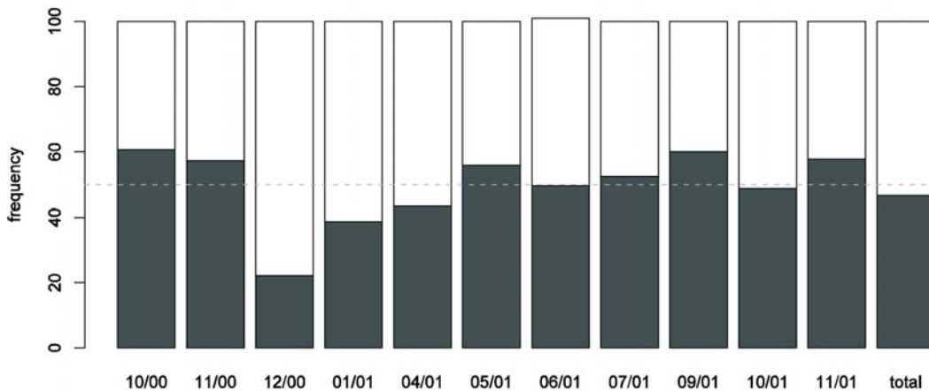
Figure 8 Variations in the sex-ratio of females (white) and males (grey) during the sampling period.
