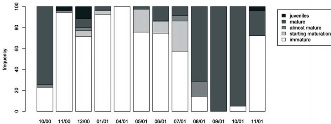
Figure 7 Internal egg stages during the sampling period.
