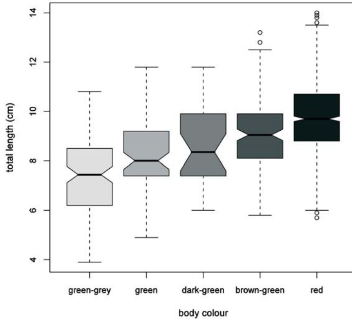
Figure 5 Boxplots of the TL separating crayfish by body colour.
