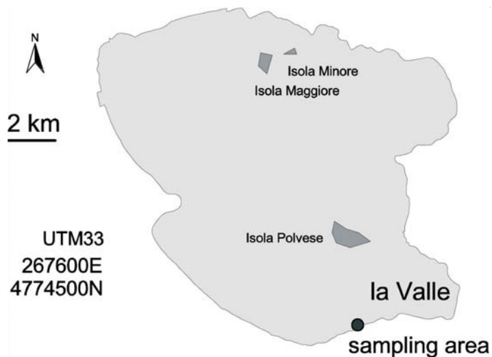
Figure 1 Lake Trasimeno. Sampling area.
