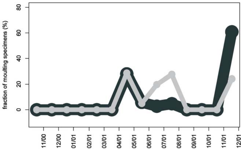
Figure 6 Fluctuation of moult for females (white) and males (grey).
