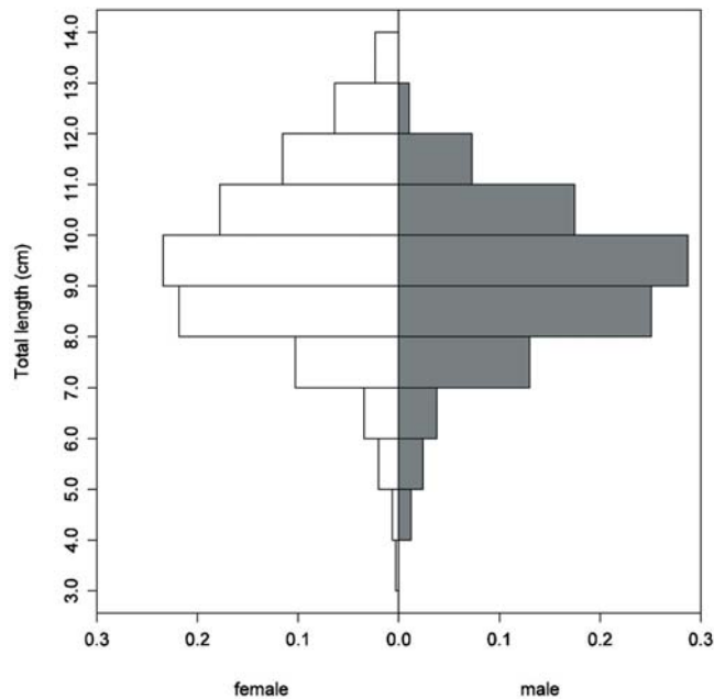
Figure 2 Frequency histogram of total lengths for males (grey) and females (white).
